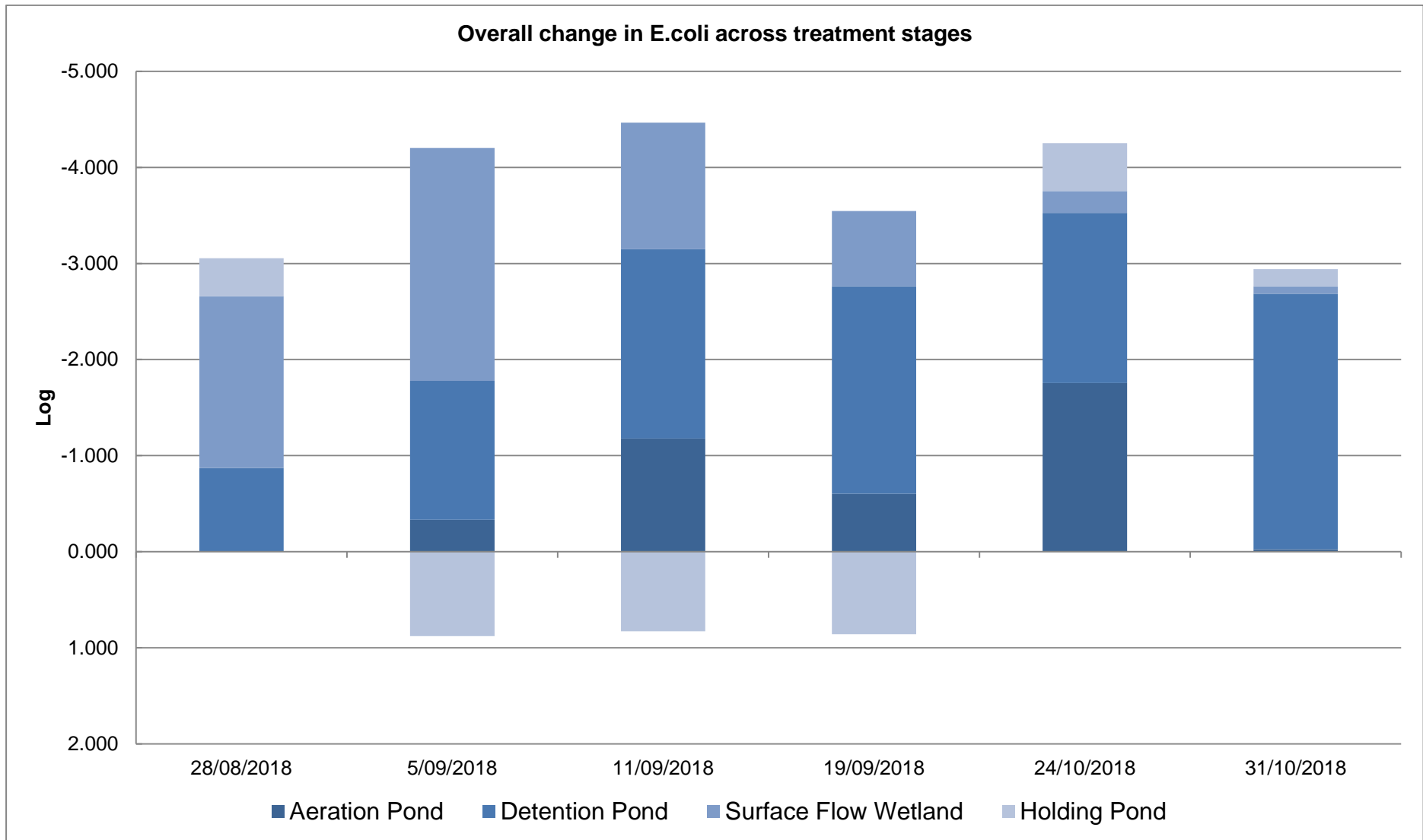
Figure 6 Overall change in E.coli counts (log) through the Opononi WWTP on 6 days of inter-stage testing.
